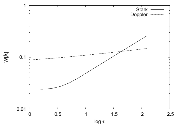
Figure 4: Stark and Doppler widths for F III 4s\ ^4P - 4p\ ^4D^o ( 8890\ \text{\AA} ) as a function of Rosseland optical depth, for an A type stellar atmosphere model with T_{eff} = 10000\ \text{K} and \log g = 4 .
