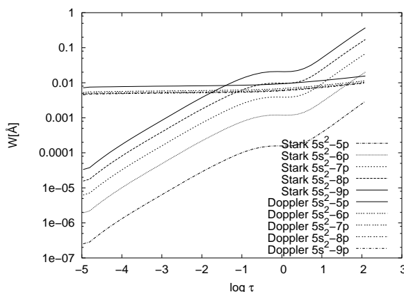
Figure 2: Thermal Doppler and Stark widths for Cd I singlet spectral lines: 5s^2\ ^1S - 5p\ ^1P^o (2288.7 Å), 5s^2\ ^1S - 6p\ ^1P^o (1669.3 Å), 5s^2\ ^1S - 7p\ ^1P^o (1526.9 Å), 5s^2\ ^1S - 8p\ ^1P^o (1469.4 Å), 5s^2\ ^1S - 9p\ ^1P^o (1440.2 Å) as a function of Rosseland optical depth.
