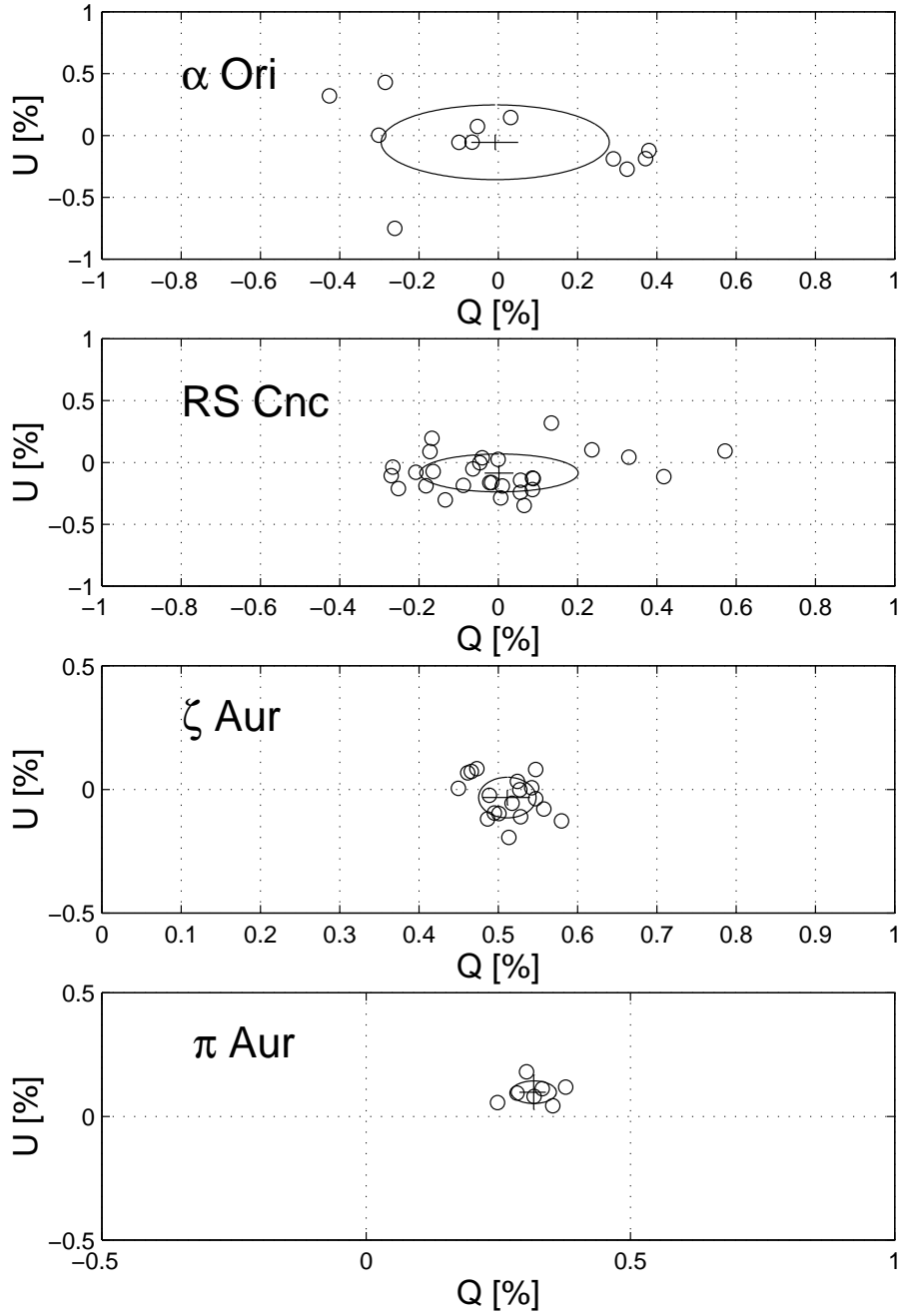
Figure 1: Median Q-U plots for the programme stars.
