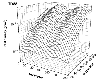
Figure 7: Dependence of the total density on the day in the year and on the flux obtained by using TD88.
