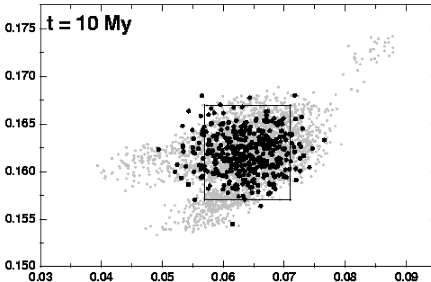
Figure 1: The snapshot in the (e_p, \sin I_p) plane, showing the spread of 400 fictitious asteroids after 10 My of evolution. The grey dots are the traces of the real resonant family members that represent the extent of the diffusive zone (as obtained after 10 My of orbit propagation, but starting from the present distribution of real family members, delimited by the box). The black dots are fictitious asteroids that evolved according to our random-walk model assuming the values of the diffusion coefficients to be as in the (5, -2, -2) region. As shown in the plot, our random-walkers cover roughly the same area as the core of the real objects. The object in the upper right corner is an escaper from the family.
