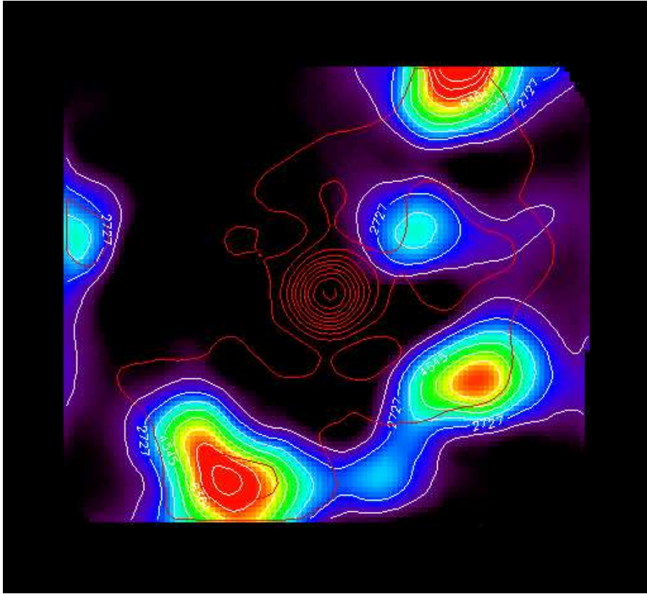
Figure 1: H\alpha map of the complex. Contours in V band are overprinted in the map indicating the position of the SMYC. Map is 32 arsec wide. North is at top and East on the left.
